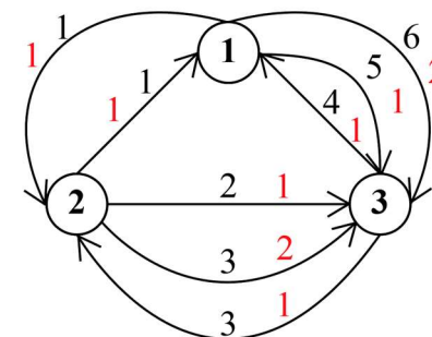
Fig. 2. The results of numbering each parallel arc
