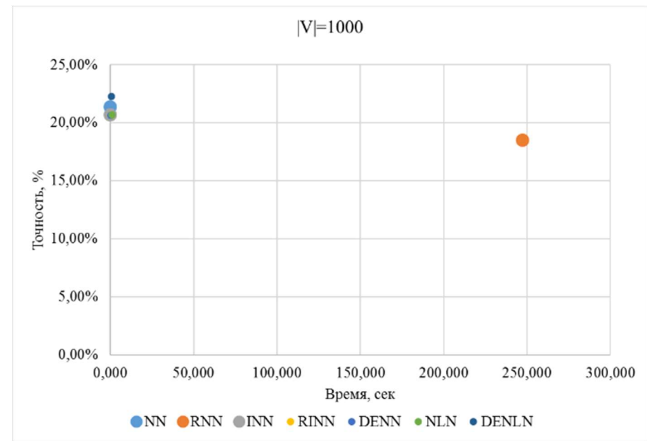
Fig. 8. The results for |V|=1000
