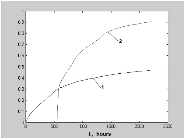
Fig.6. Characteristics of efficiency of oil recovery. Line 1 - \theta(t) , line 2 - \gamma(t) . k_{D1} = 0.50 \cdot 10^{-12} m^2 .
