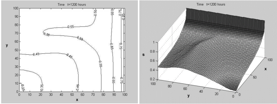
Fig.5. The water saturation at t = 1200 hours. k_{D1} = 0.50 \cdot 10^{-12} m^2 .
