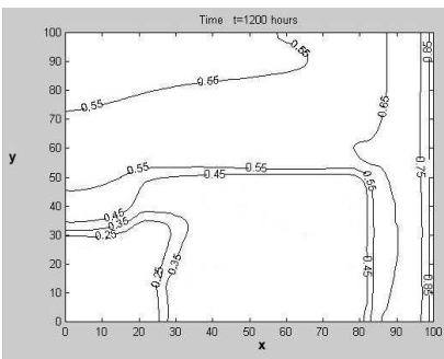
Fig.9. The water saturation at t = 1200 hours. k_{D1} = 0.20 \cdot 10^{-12} \text{ m}^2 .
