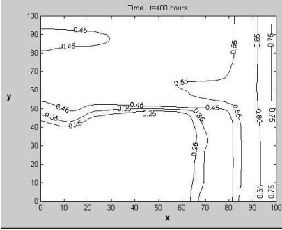
Fig.7. The water saturation at t = 400 hours. k_{D1} = 0.20 \cdot 10^{-12} \text{ m}^2 .
