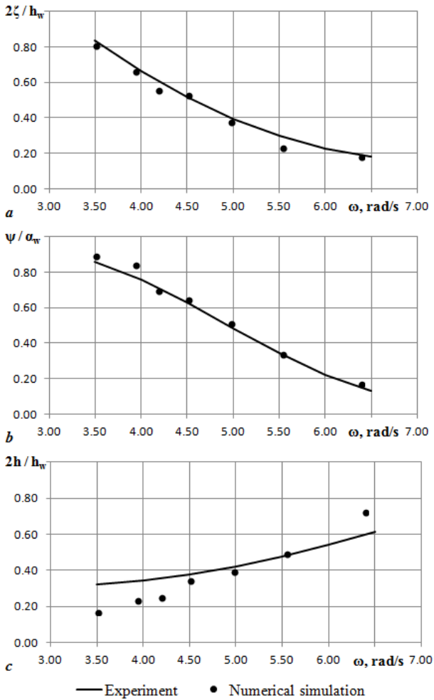
Fig. 12. RAO of heave (a) and pitch (b) motions and vertical water motions in the moonpool (c) of the model with module No. 2.
