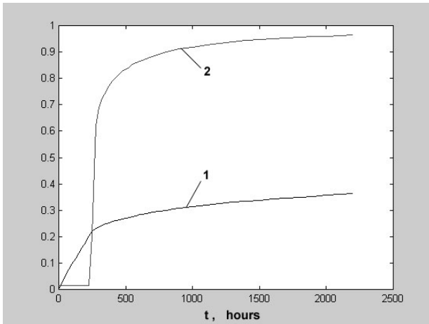
Fig.14. Characteristics of efficiency of oil recovery. Line 1 - \theta(t) , line 2 - \gamma(t) . k_{D1} = 0.01 \cdot 10^{-12} m^2 .
