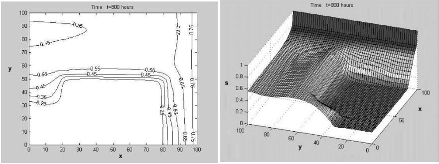
Fig.12. The water saturation at t = 800 hours. k_{D1} = 0.01 \cdot 10^{-12} m^2 .
