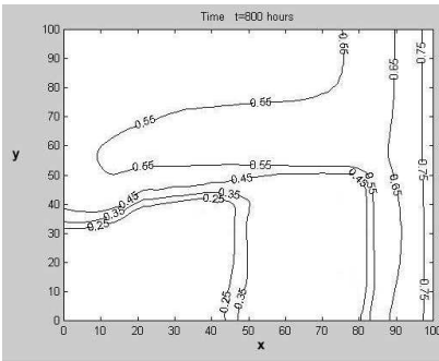
Fig.8. The water saturation at t = 800 hours. k_{D1} = 0.20 \cdot 10^{-12} \text{ m}^2 .
