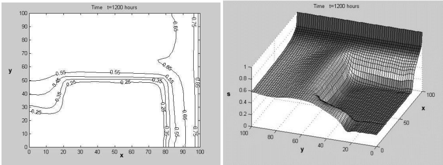
Fig.13. The water saturation at t = 1200 hours. k_{D1} = 0.01 \cdot 10^{-12} m^2 .
