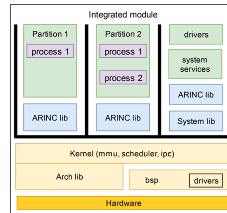
Fig. 3. JetOS architecture
