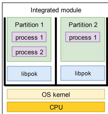
Fig. 2. POK architecture
